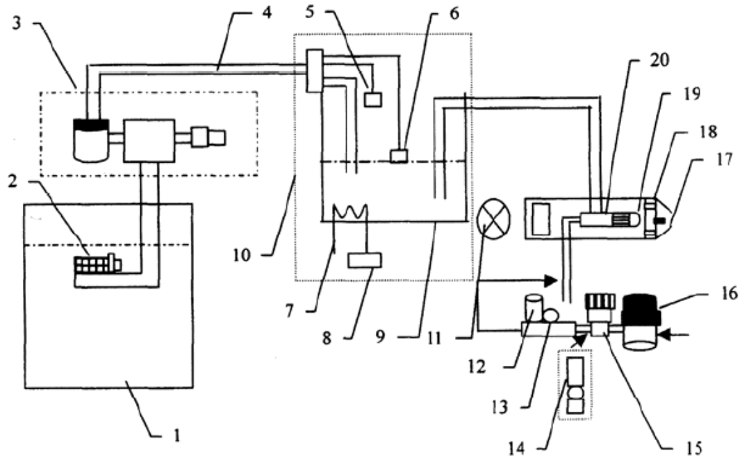
Fig 1 Air and Fuel Oil Flow Chart
